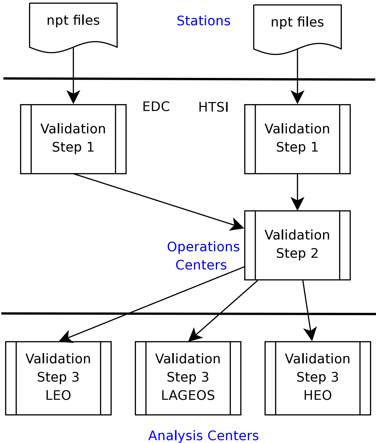
CRD Data Validation Flow
