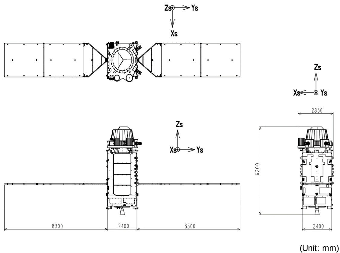
Figure 4 Satellite dimensions
