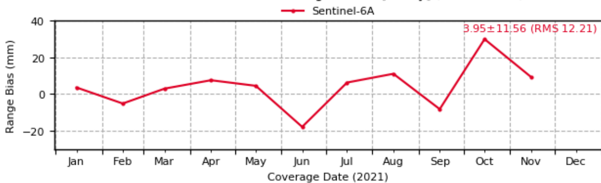
Sentinel-6: Evolution of Range Biases [1-way] (1893 - KTZL)
