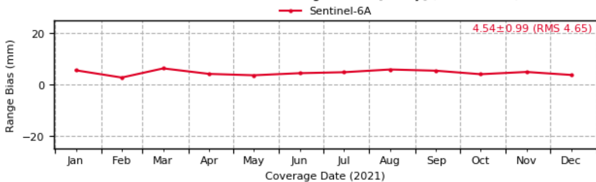
Sentinel-6: Evolution of Range Biases [1-way] (7090 - YARL)
