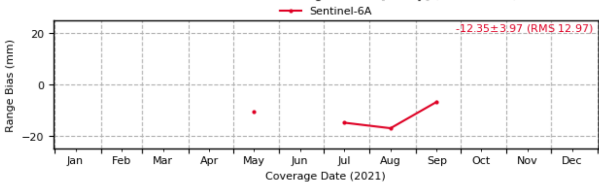
Sentinel-6: Evolution of Range Biases [1-way] (7249 - BEIL)
