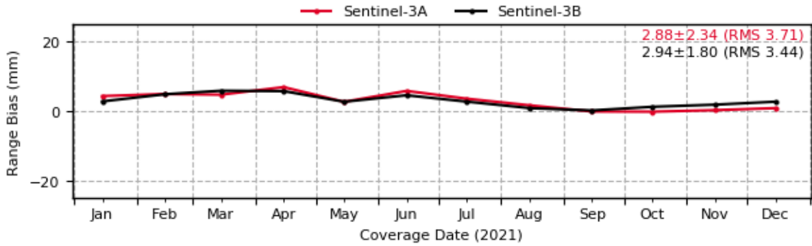
Sentinel-3: Evolution of Range Biases [1-way] (7110 - MONL)
