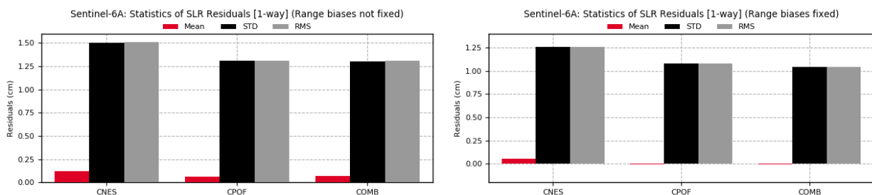
Figure 3-19: Mean, STD and RMS of the Sentinel-6A SLR observation residuals [1-way; cm] from all orbit solutions in 2021 (left the range biases have not been fixed, right the range biases have been fixed)
