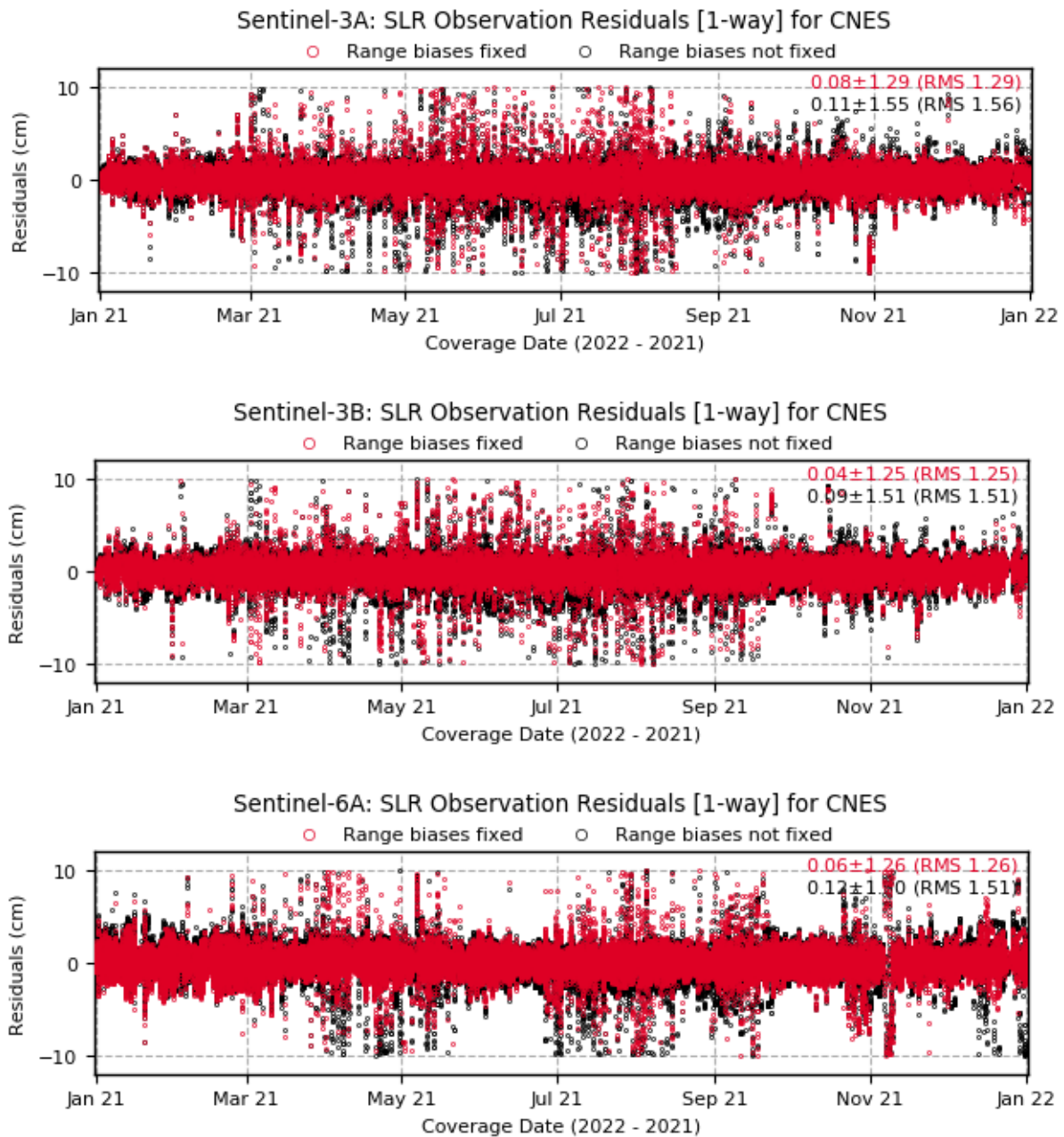
Figure 3-14: SLR observation residuals [1-way; cm] obtained for CNES orbit solution in 2021 (Sentinel-3A, Sentinel-3B and Sentinel-6A)
