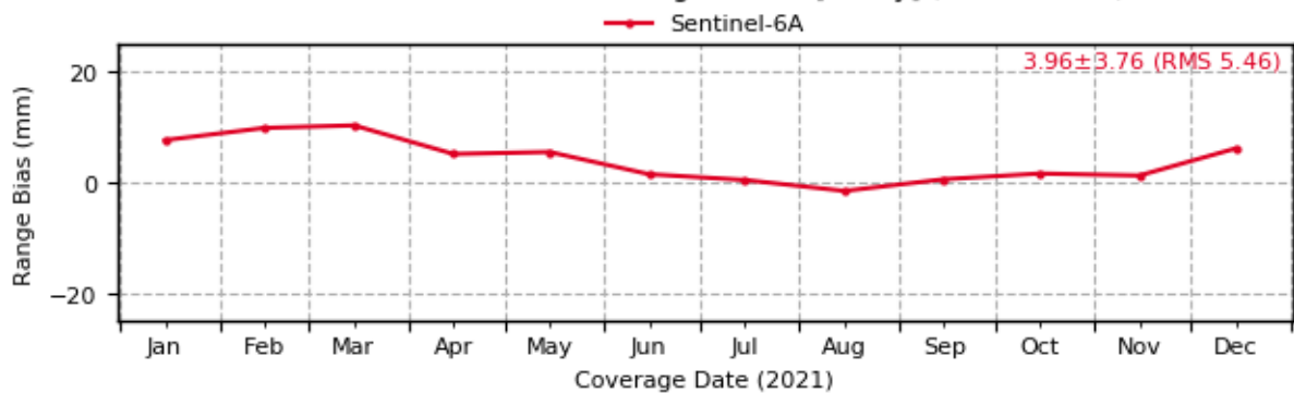
Sentinel-6: Evolution of Range Biases [1-way] (7839 - GRZL)
