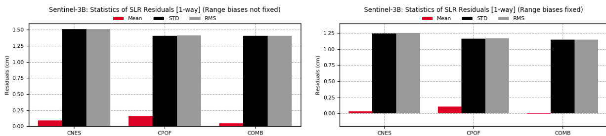
Figure 3-18: Mean, STD and RMS of the Sentinel-3B SLR observation residuals [1-way; cm] from all orbit solutions in 2021 (left the range biases have not been fixed, right the range biases have been fixed)
