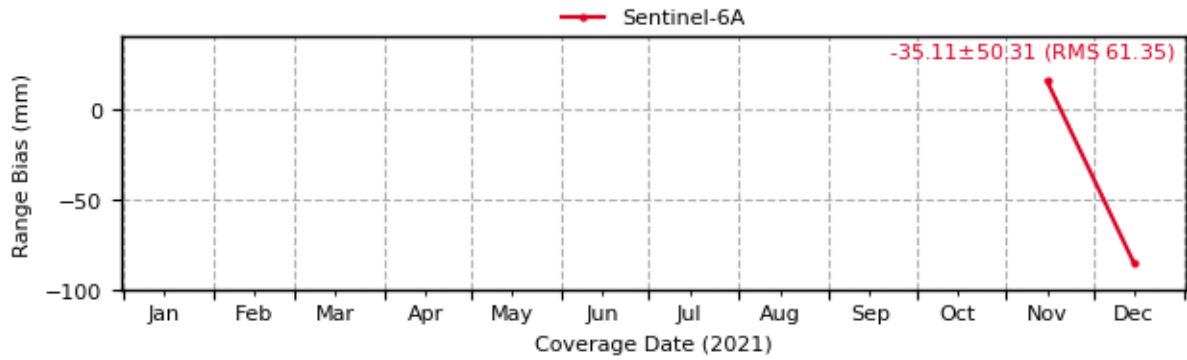
Sentinel-6: Evolution of Range Biases [1-way] (7819 - KUN2)
