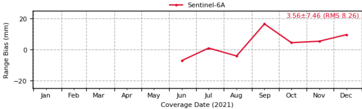
Sentinel-6: Evolution of Range Biases [1-way] (7396 - JFNL)
