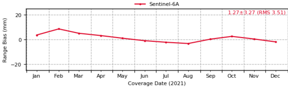
Sentinel-6: Evolution of Range Biases [1-way] (7840 - HERL)
