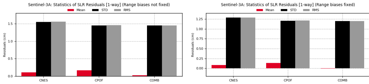
Figure 3-17: Mean, STD and RMS of the Sentinel-3A SLR observation residuals [1-way; cm] from all orbit solutions in 2021 (left the range biases have not been fixed, right the range biases have been fixed)
