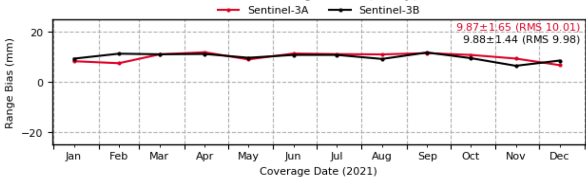
Sentinel-3: Evolution of Range Biases [1-way] (7119 - HA4T)
