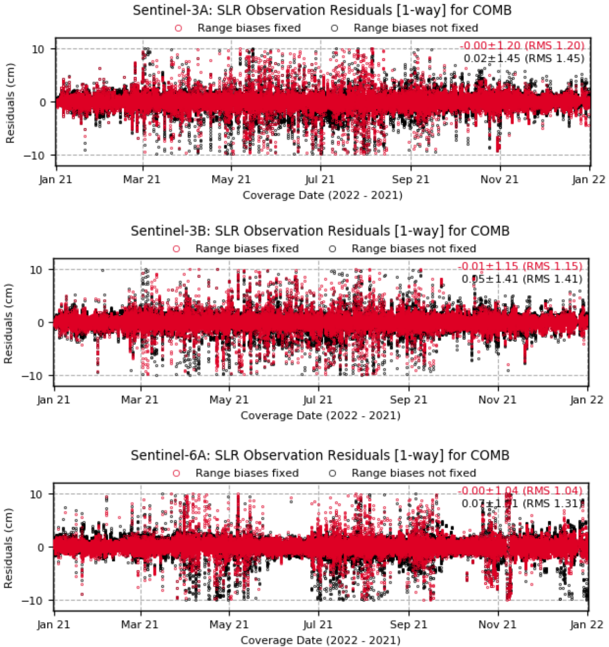
Figure 3-16: SLR observation residuals [1-way; cm] obtained for COMB orbit solution in 2021 (Sentinel-3A, Sentinel-3B and Sentinel-6A)
