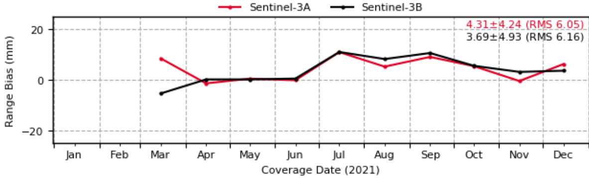
Sentinel-3: Evolution of Range Biases [1-way] (7501 - HARL)
