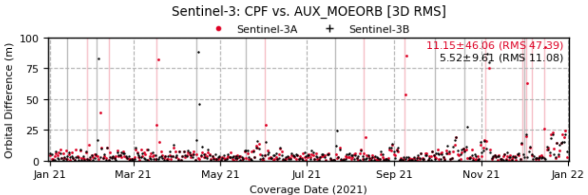
Figure 4-1: Orbital comparisons [3D RMS; m] between the Sentinel-3 CPF predictions and the Sentinel-3 CPOD STC products during 2021
