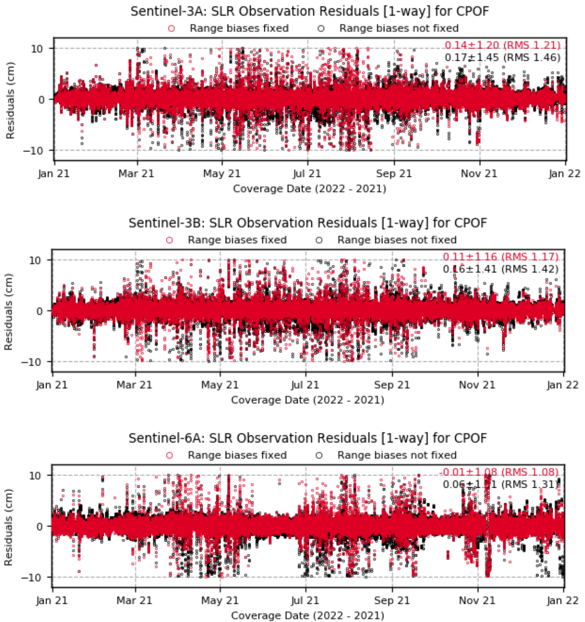
Figure 3-15: SLR observation residuals [1-way; cm] obtained for CPOF orbit solution in 2021 (Sentinel-3A, Sentinel-3B and Sentinel-6A)
