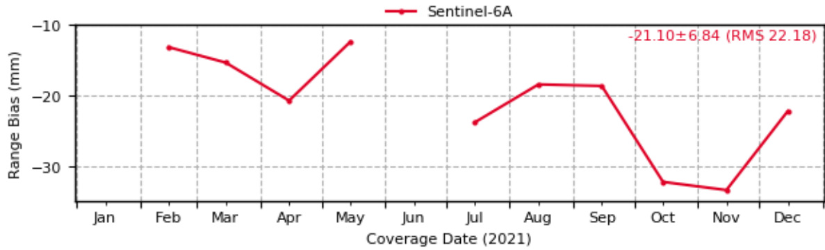
Sentinel-6: Evolution of Range Biases [1-way] (7811 - BORL)
