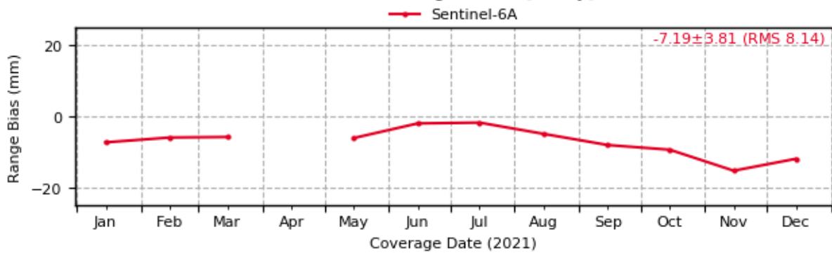
Sentinel-6: Evolution of Range Biases [1-way] (7403 - AREL)
