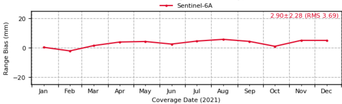
Sentinel-6: Evolution of Range Biases [1-way] (7825 - STL3)
