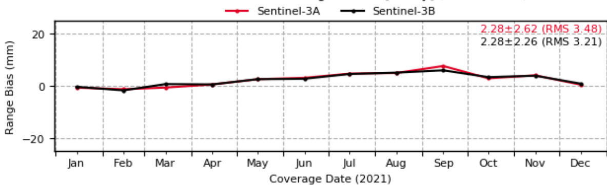
Sentinel-3: Evolution of Range Biases [1-way] (7825 - STL3)
