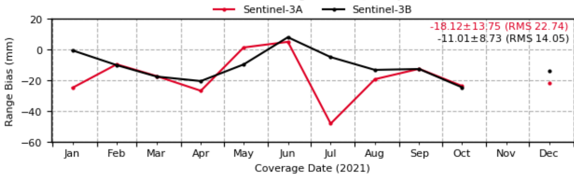
Sentinel-3: Evolution of Range Biases [1-way] (7811 - BORL)
