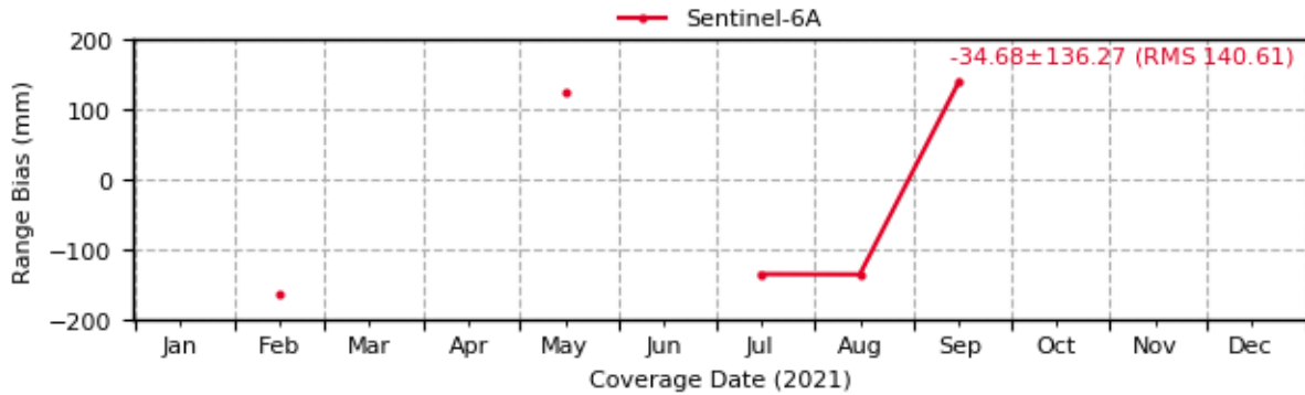
Sentinel-6: Evolution of Range Biases [1-way] (1824 - GLSL)
