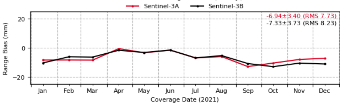
Sentinel-3: Evolution of Range Biases [1-way] (7403 - AREL)
