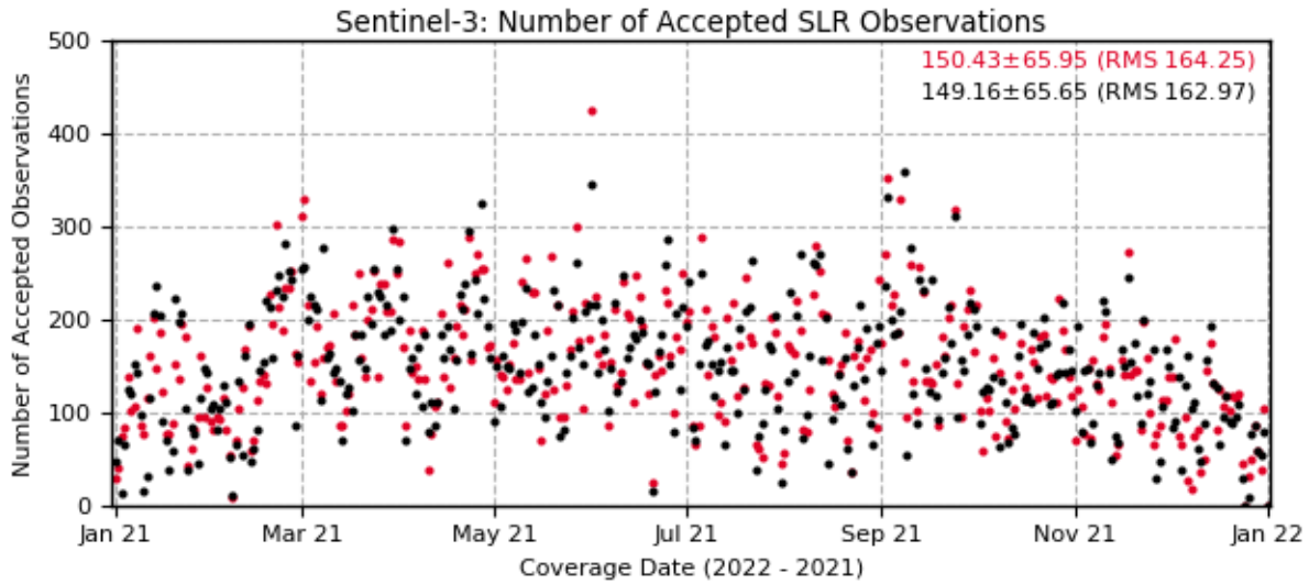
Figure 3-7: Daily total number of the accepted SLR observations of all SLR stations tracking Sentinel-3A and Sentinel-3B satellites in 2021
