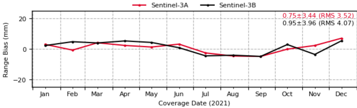
Sentinel-3: Evolution of Range Biases [1-way] (7810 - ZIML)
