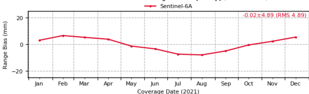
Sentinel-6: Evolution of Range Biases [1-way] (7810 - ZIML)
