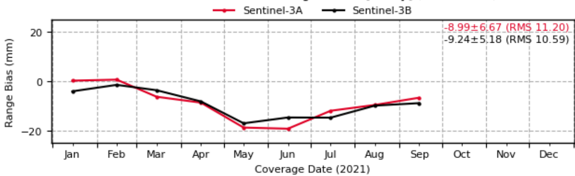
Sentinel-3: Evolution of Range Biases [1-way] (7249 - BEIL)
