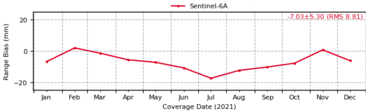
Sentinel-6: Evolution of Range Biases [1-way] (7841 - POT3)
