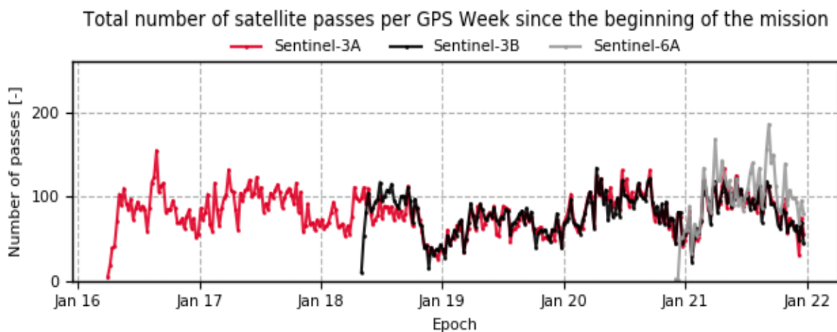
Figure 2-5: Total number of satellite passes per GPS week since the beginning of the satellite mission (Sentinel-3A, Sentinel-3B and Sentinel-6A)
