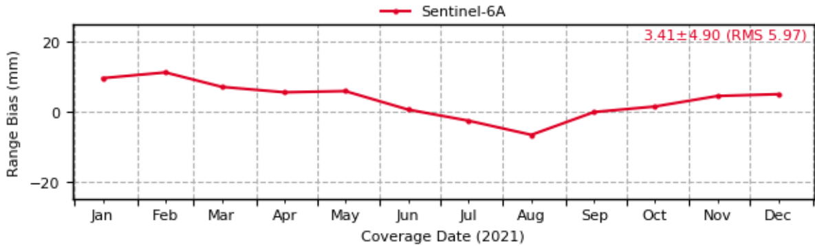
Sentinel-6: Evolution of Range Biases [1-way] (7105 - GODL)
