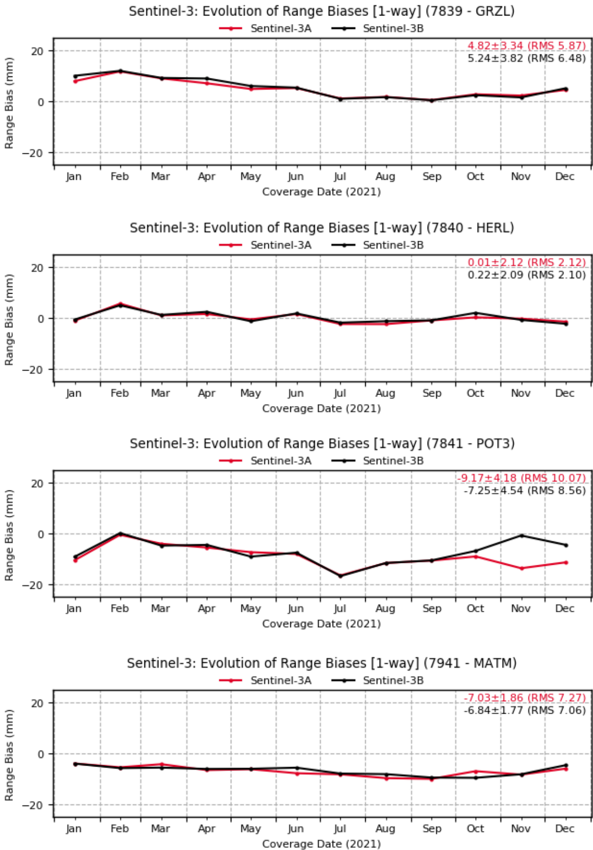
Figure 3-9: Evolution of the range biases [1-way; mm] calculated for each SLR station tracking Sentinel-3A and Sentinel-3B satellites in 2021
