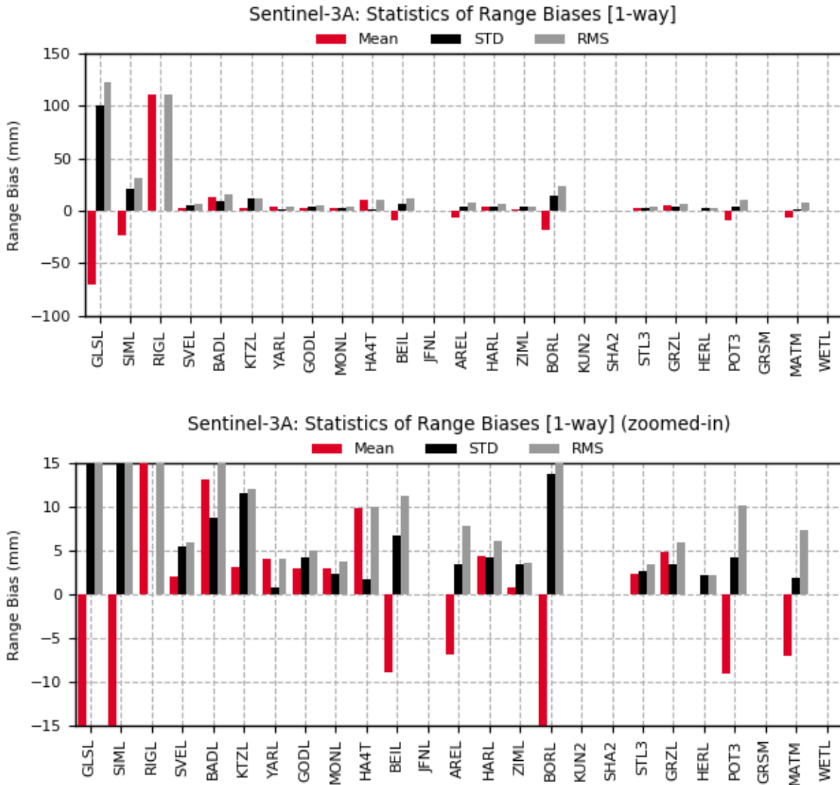
Figure 3-11: Mean, STD and RMS of the Sentinel-3A range biases [1-way; mm] of each SLR station (the figure below is a zoomed-in of the figure above)
