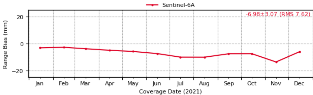
Sentinel-6: Evolution of Range Biases [1-way] (7941 - MATM)
