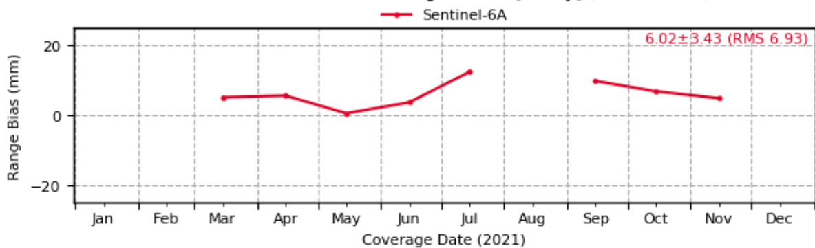
Sentinel-6: Evolution of Range Biases [1-way] (7501 - HARL)
