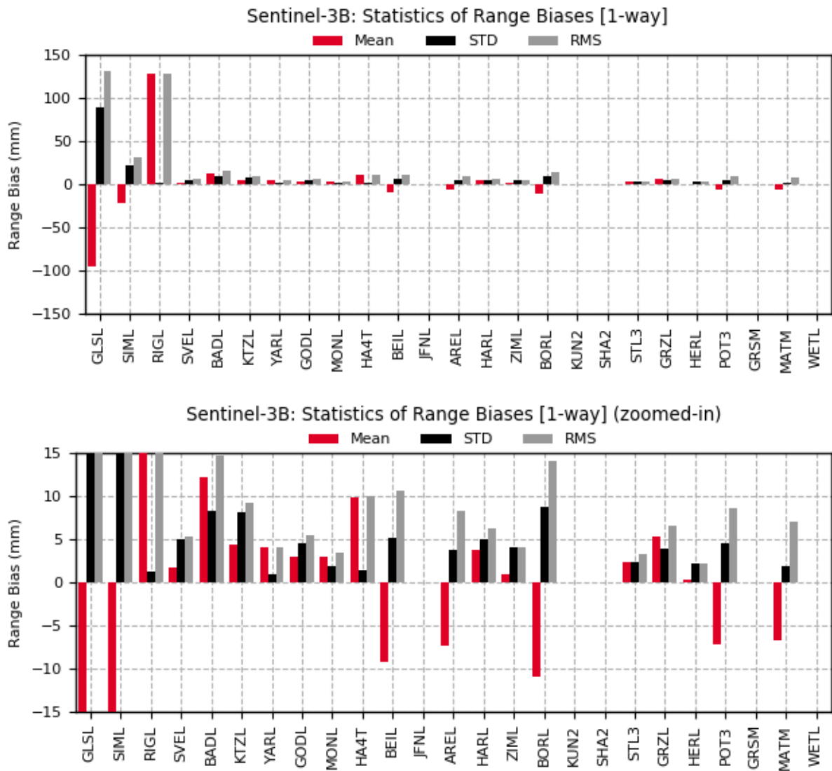
Figure 3-12: Mean, STD and RMS of the Sentinel-3B range biases [1-way; mm] of each SLR station (the figure below is a zoomed-in of the figure above)
