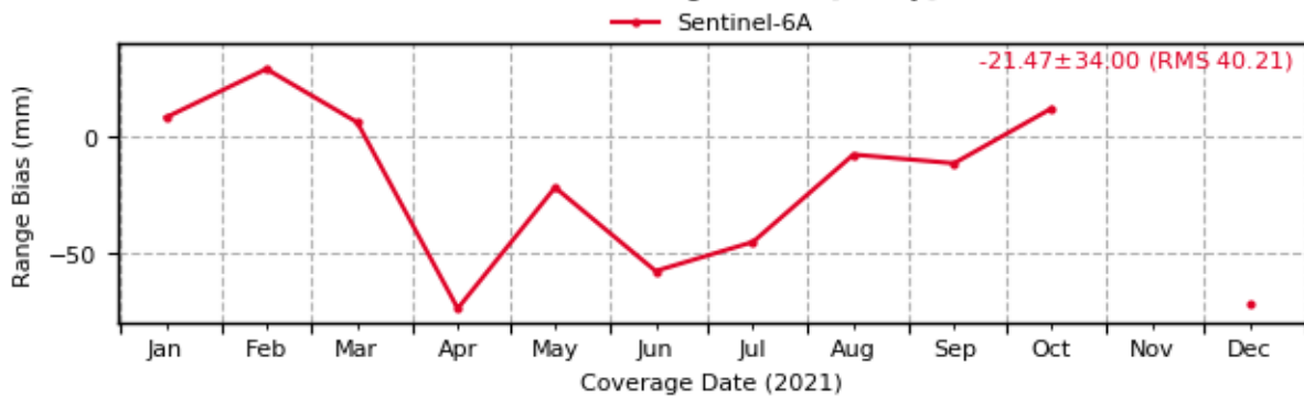
Sentinel-6: Evolution of Range Biases [1-way] (1873 - SIML)
