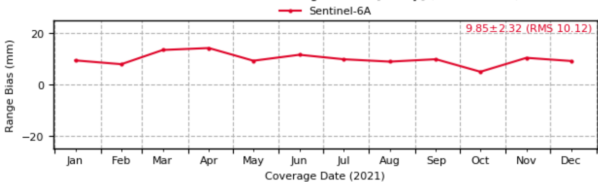
Sentinel-6: Evolution of Range Biases [1-way] (7119 - HA4T)
