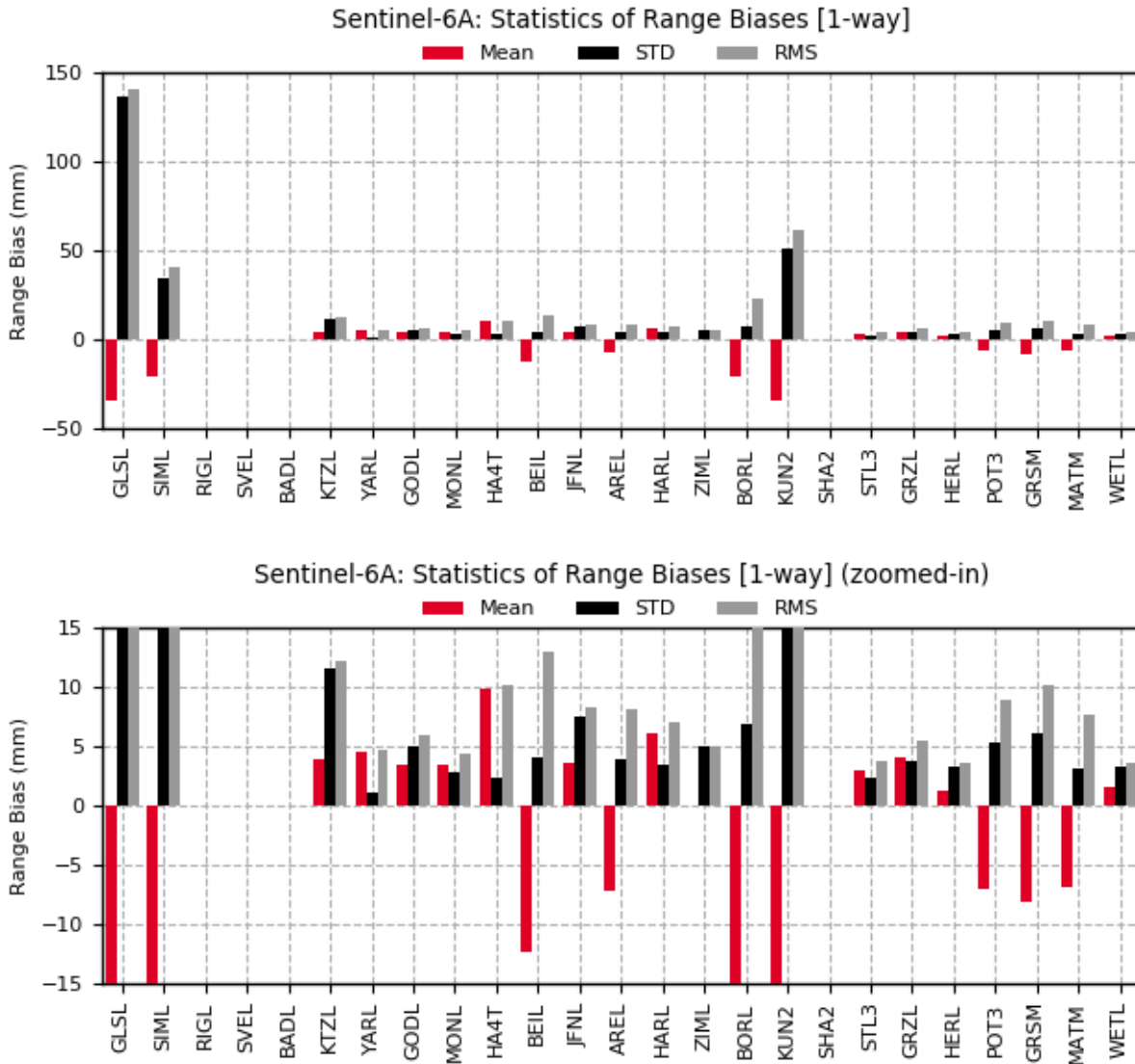
Figure 3-13: Mean, STD and RMS of the Sentinel-6A range biases [1-way; mm] of each SLR station (the figure below is a zoomed-in of the figure above)
