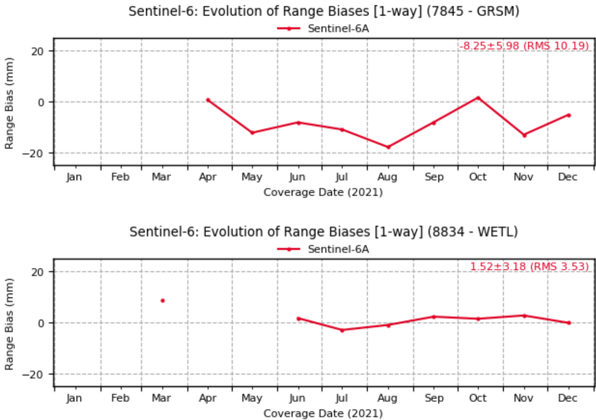
Figure 3-10: Evolution of the range biases [1-way; mm] calculated for each SLR station tracking Sentinel-6A satellite in 2021
