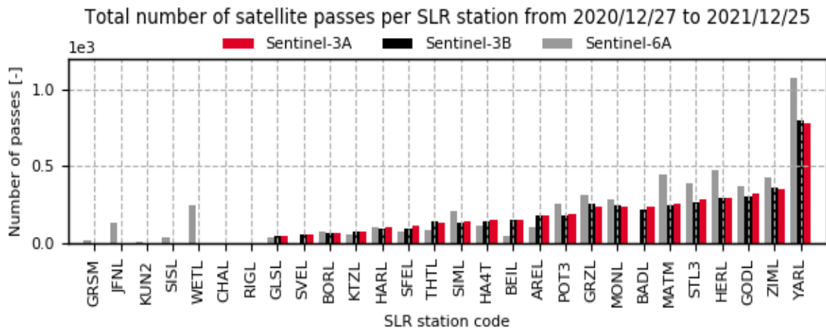
Figure 2-8: Total number of satellite passes per SLR station in 2021 (Sentinel-3A, Sentinel-3B and Sentinel-6A)
