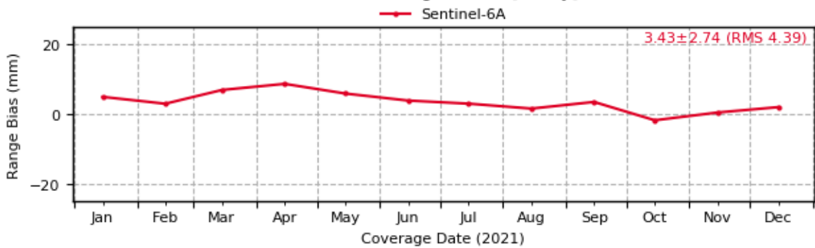
Sentinel-6: Evolution of Range Biases [1-way] (7110 - MONL)
