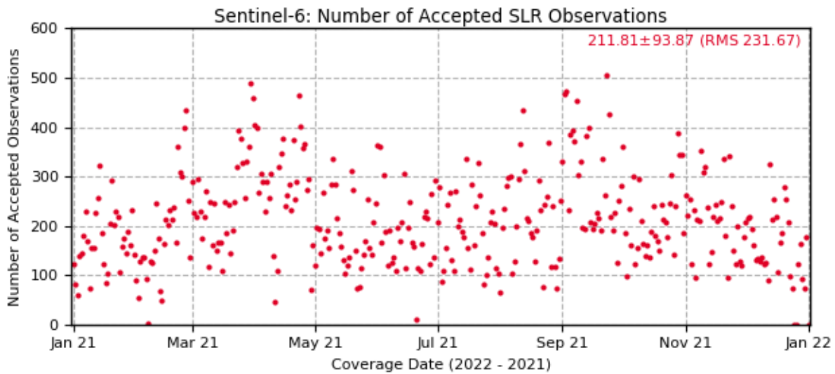
Figure 3-8: Daily total number of the accepted SLR observations of all SLR stations tracking Sentinel-6A satellite in 2021
