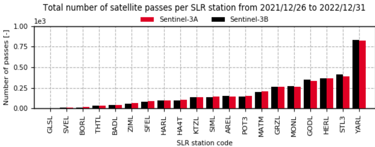
Figure 2-10: Total number of satellite passes per SLR station in 2022 (Sentinel-3A and Sentinel-3B)
