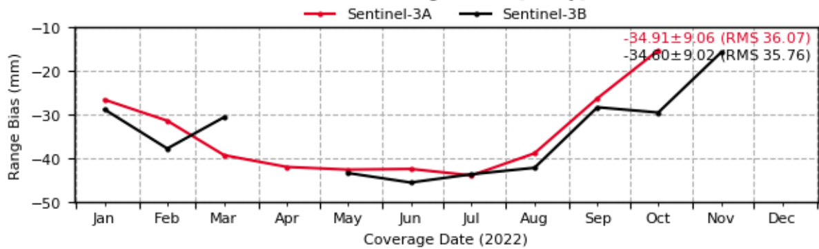
Sentinel-3: Evolution of Range Biases [1-way] (7824 - SFEL)
