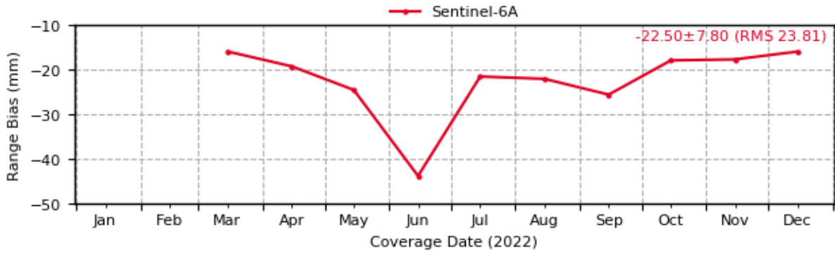
Sentinel-6: Evolution of Range Biases [1-way] (7237 - CHAL)
