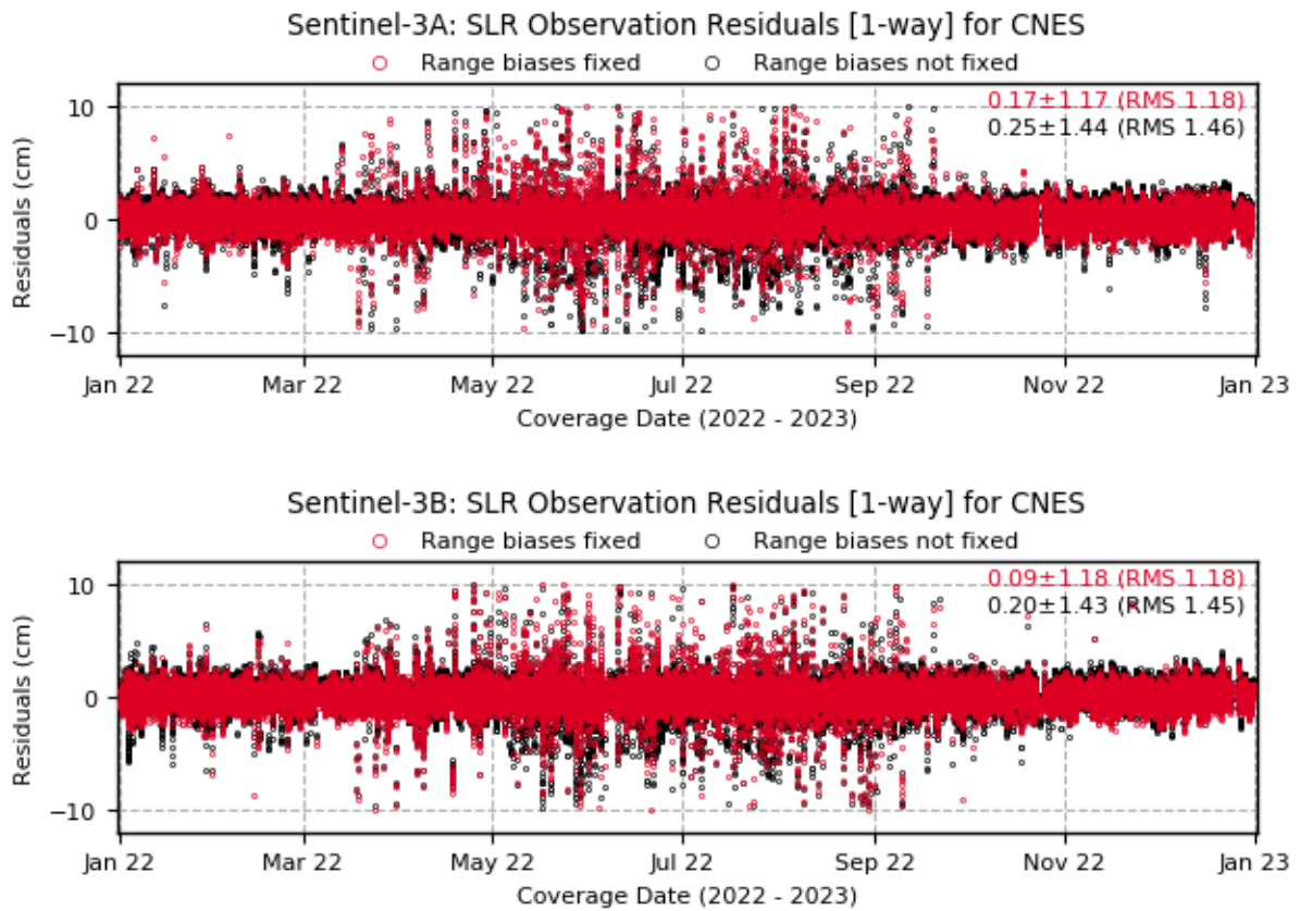
Figure 3-14: SLR observation residuals [1-way; cm] obtained for CNES orbit solution in 2022 (above Sentinel-3A, and below Sentinel-3B)
