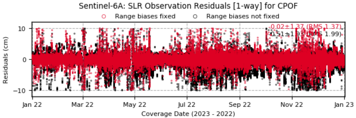
Figure 3-18: SLR observation residuals [1-way; cm] obtained for CPOF orbit solution in 2022 (Sentinel-6A)
