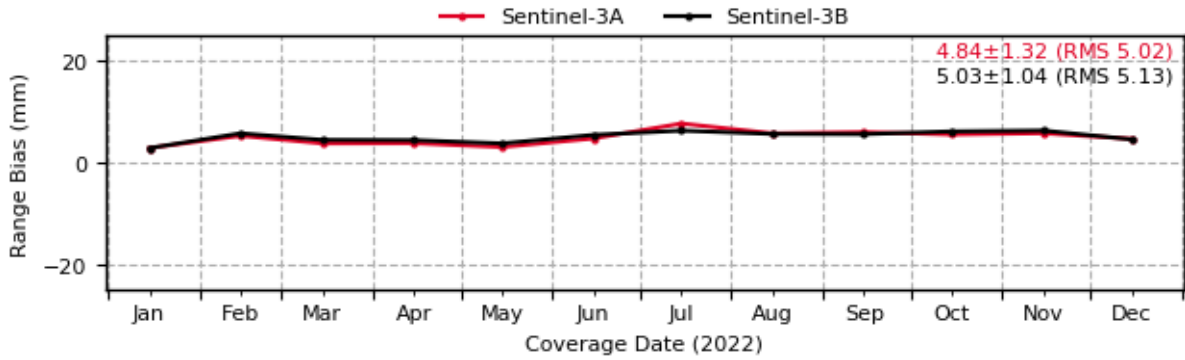
Sentinel-3: Evolution of Range Biases [1-way] (7090 - YARL)
