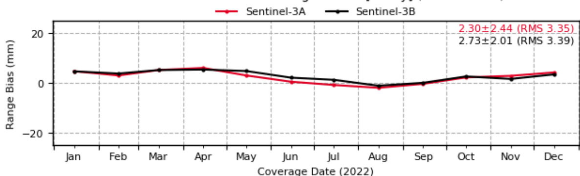
Sentinel-3: Evolution of Range Biases [1-way] (7839 - GRZL)
