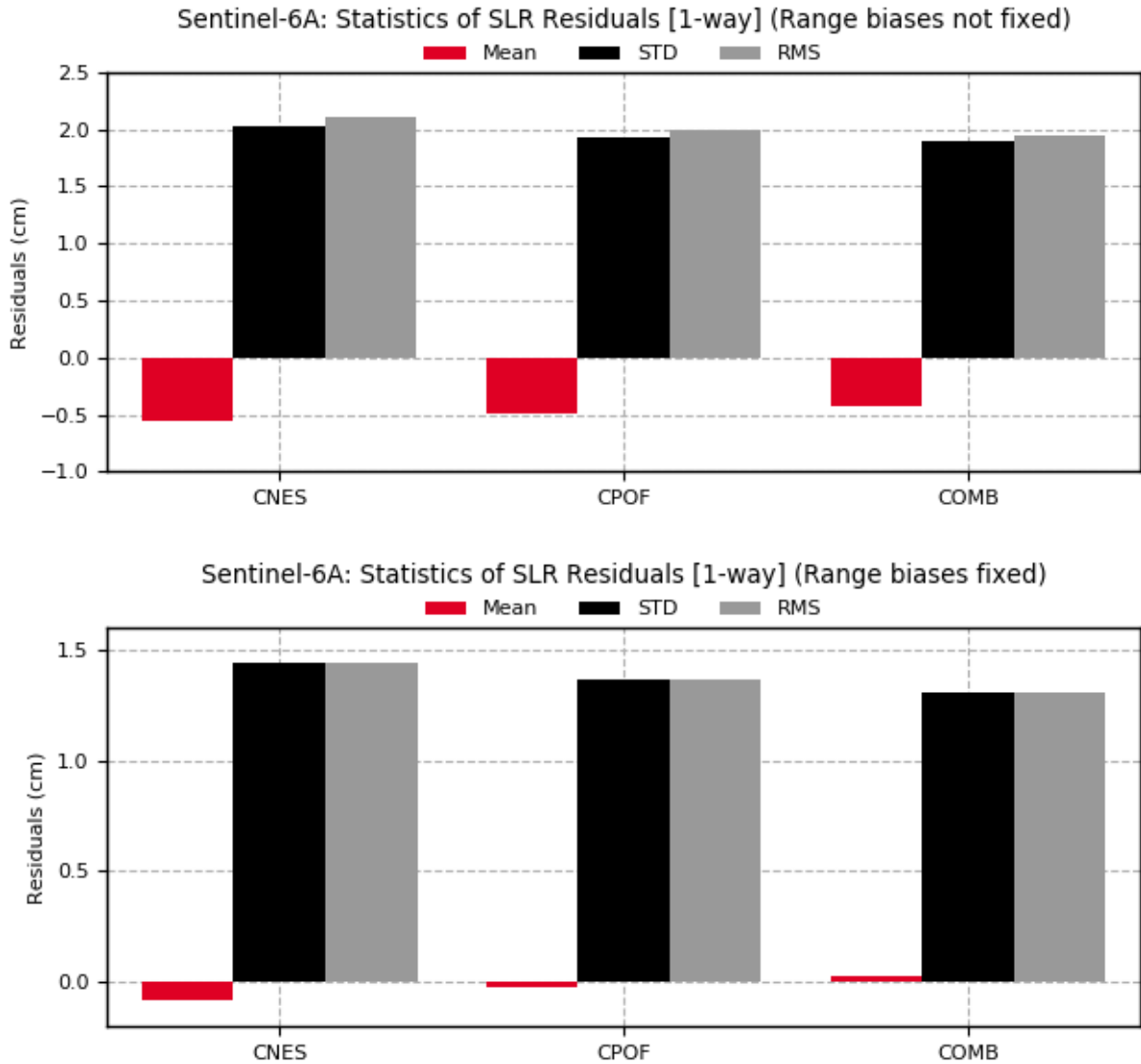
Figure 3-22: Mean, STD and RMS of the Sentinel-6A SLR observation residuals [1-way; cm] from all orbit solutions in 2022 (above the range biases have not been fixed, below the range biases have been fixed)
