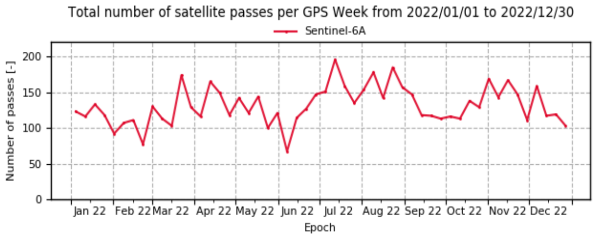
Figure 2-8: Total number of satellite passes per GPS week in 2022 (Sentinel-6A)
