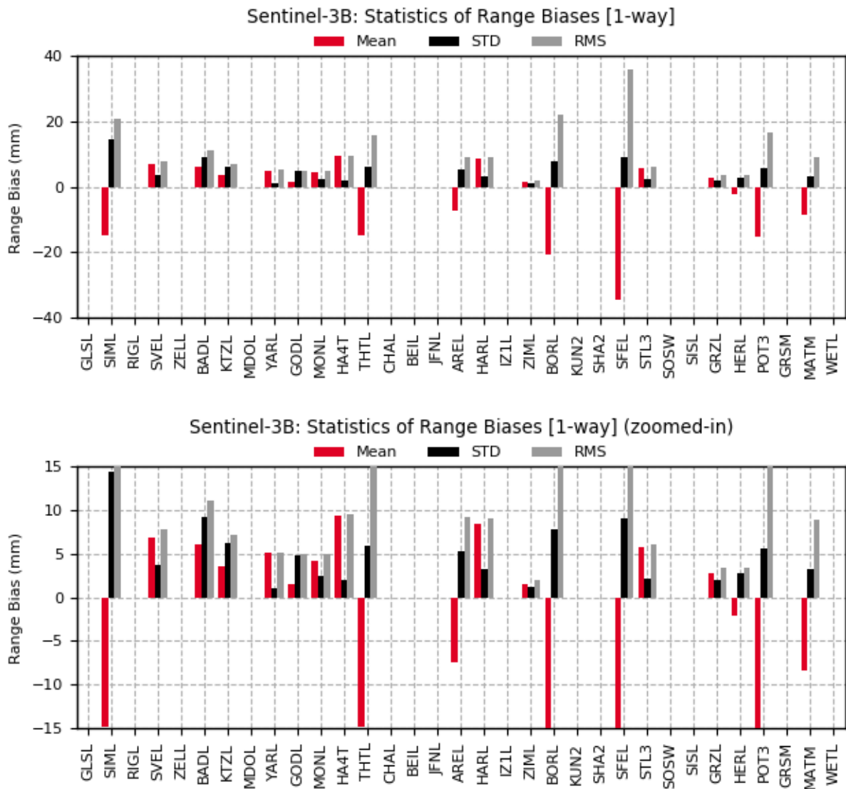
Figure 3-12: Mean, STD and RMS of the Sentinel-3B range biases [1-way; mm] of each SLR station (the figure below is a zoomed-in of the figure above)
