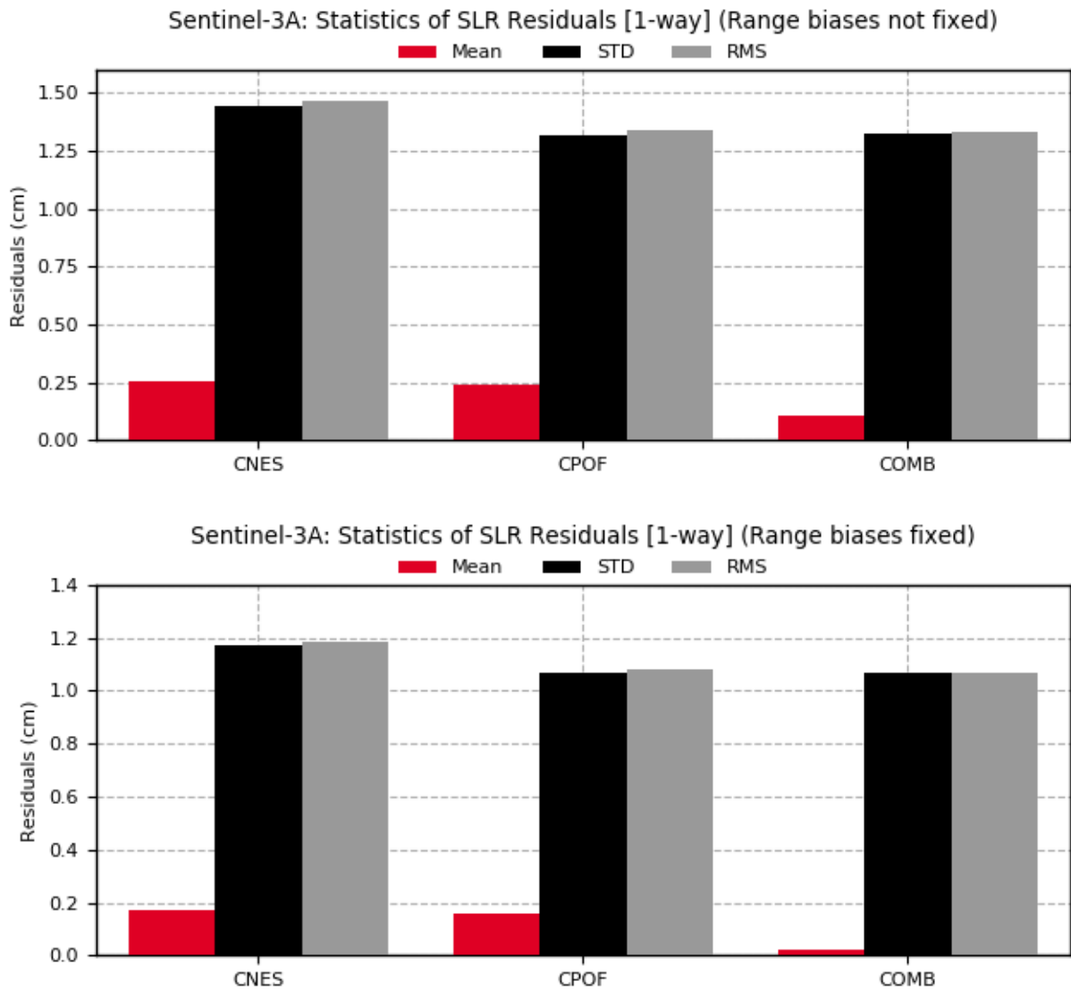
Figure 3-20: Mean, STD and RMS of the Sentinel-3A SLR observation residuals [1-way; cm] from all orbit solutions in 2022 (above the range biases have not been fixed, below the range biases have been fixed)
