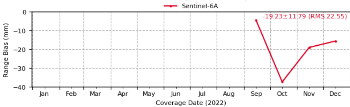
Sentinel-6: Evolution of Range Biases [1-way] (7701 - IZ1L)
