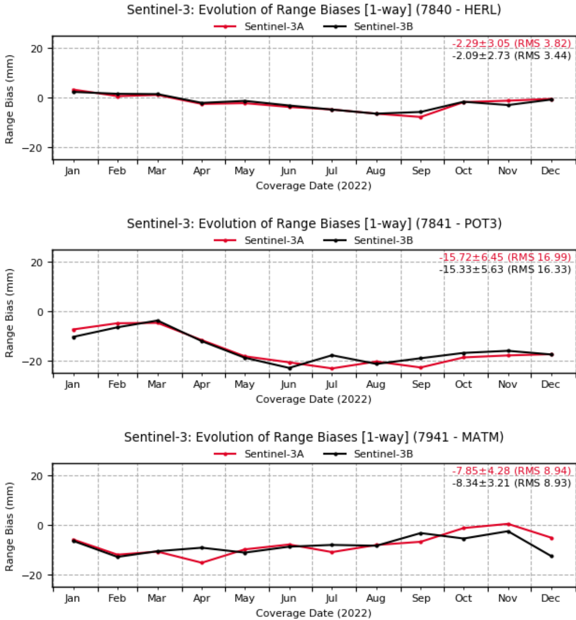
Figure 3-9: Evolution of the range biases [1-way; mm] calculated for each SLR station tracking Sentinel-3A and Sentinel-3B satellites in 2022
