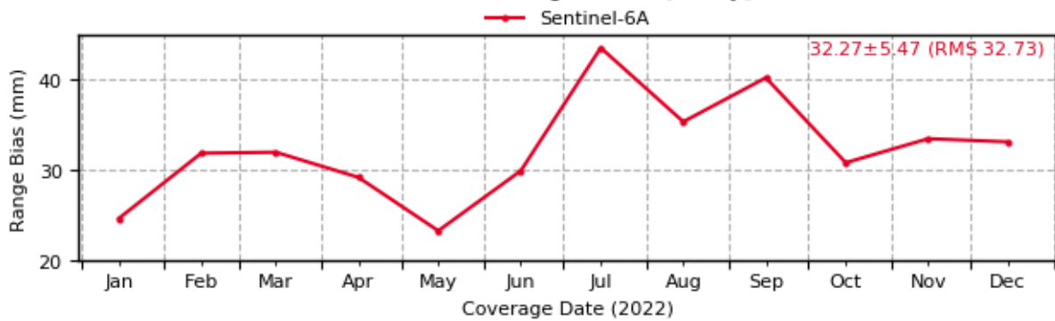
Sentinel-6: Evolution of Range Biases [1-way] (7838 - SISL)
