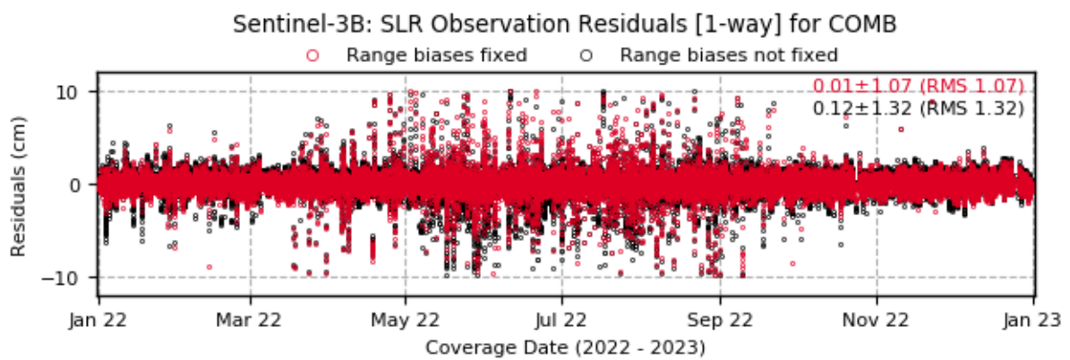
Figure 3-16: SLR observation residuals [1-way; cm] obtained for COMB orbit solution in 2022 (above Sentinel-3A, and below Sentinel-3B)
