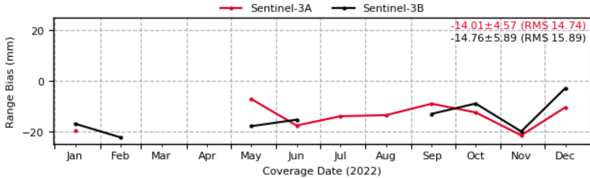
Sentinel-3: Evolution of Range Biases [1-way] (7124 - THTL)
