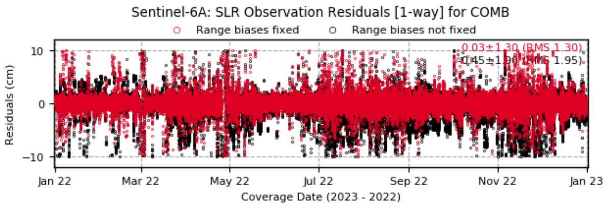
Figure 3-19: SLR observation residuals [1-way; cm] obtained for COMB orbit solution in 2022 (Sentinel-6A)
