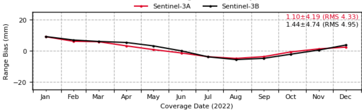
Sentinel-3: Evolution of Range Biases [1-way] (7105 - GODL)
