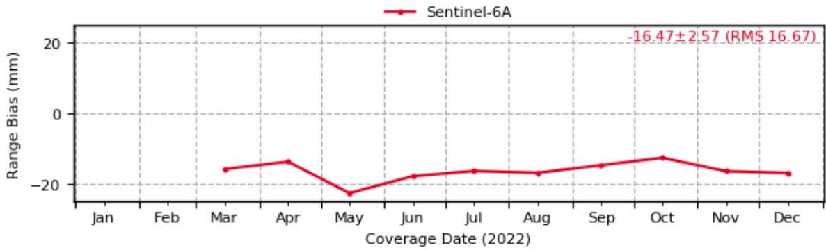
Sentinel-6: Evolution of Range Biases [1-way] (7821 - SHA2)
