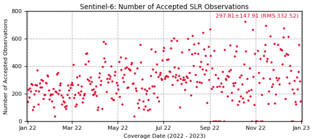
Figure 3-8: Daily total number of the accepted SLR observations of all SLR stations tracking Sentinel-6A satellite in 2022
