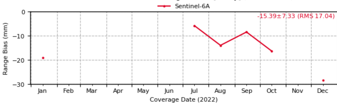
Sentinel-6: Evolution of Range Biases [1-way] (7124 - THTL)
