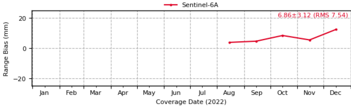
Sentinel-6: Evolution of Range Biases [1-way] (7827 - SOSW)
