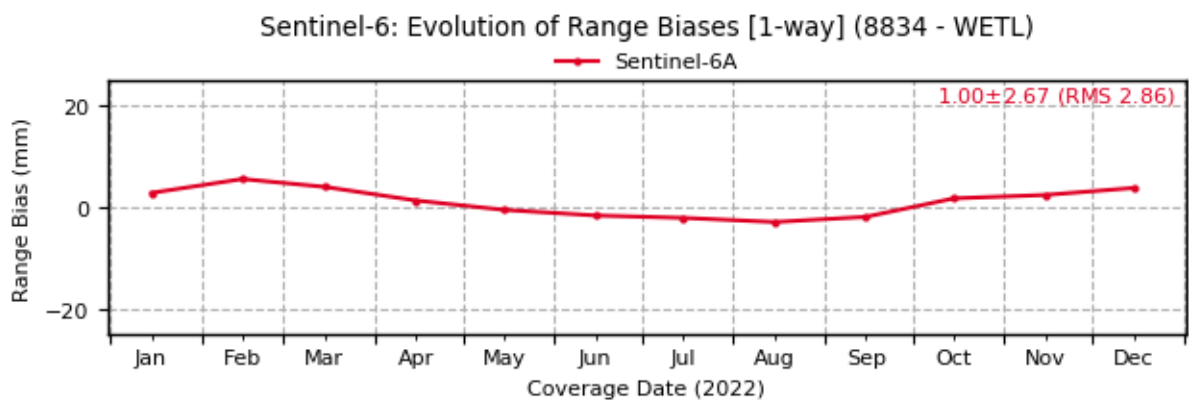
Figure 3-10: Evolution of the range biases [1-way; mm] calculated for each SLR station tracking Sentinel-6A satellite in 2022
