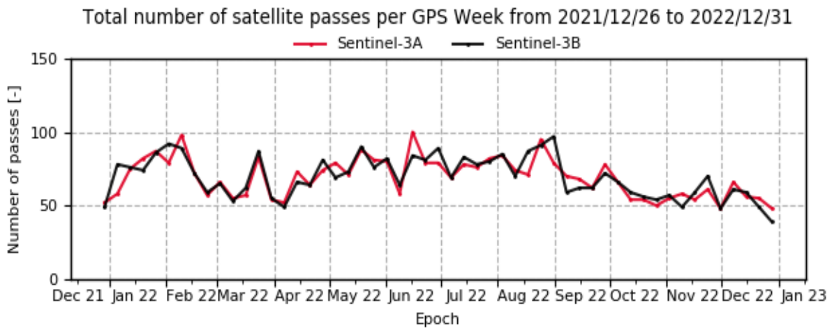
Figure 2-6: Total number of satellite passes per GPS week in 2022 (Sentinel-3A and Sentinel-3B)
