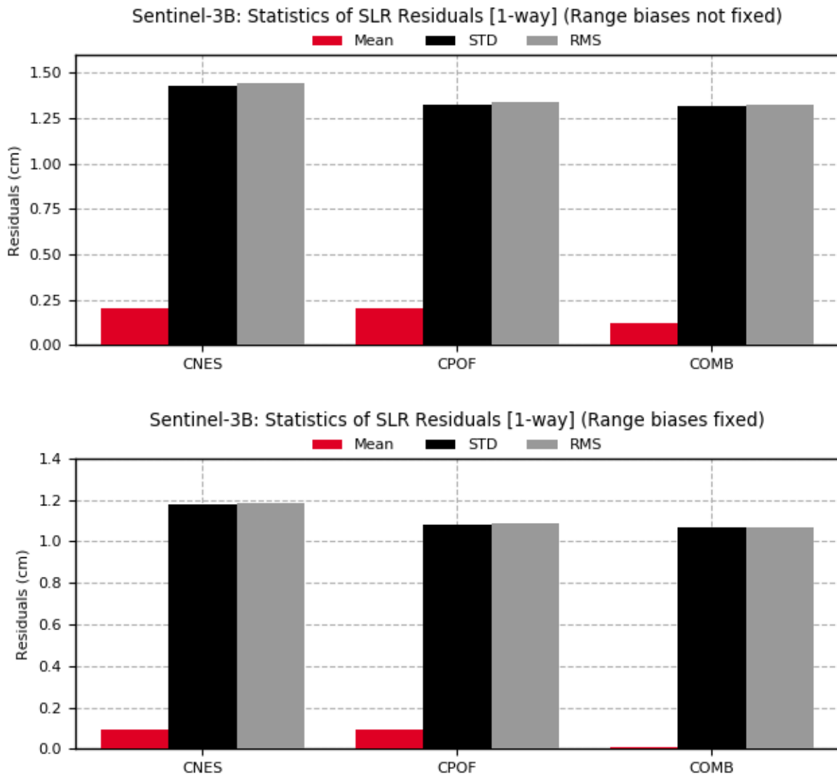
Figure 3-21: Mean, STD and RMS of the Sentinel-3B SLR observation residuals [1-way; cm] from all orbit solutions in 2022 (above the range biases have not been fixed, below the range biases have been fixed)
