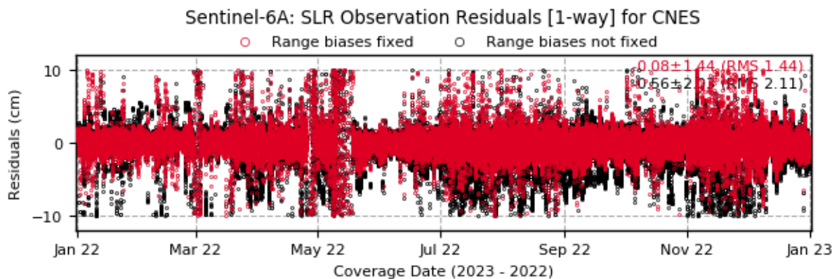
Figure 3-17: SLR observation residuals [1-way; cm] obtained for CNES orbit solution in 2022 (Sentinel-6A)
