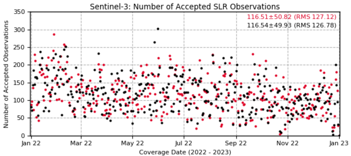
Figure 3-7: Daily total number of the accepted SLR observations of all SLR stations tracking Sentinel-3A and Sentinel-3B satellites in 2022
