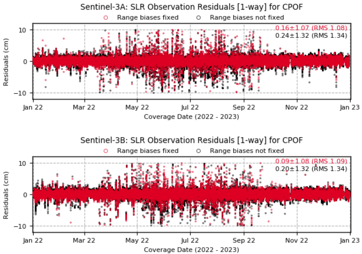
Figure 3-15: SLR observation residuals [1-way; cm] obtained for CPOF orbit solution in 2022 (above Sentinel-3A, and below Sentinel-3B)
