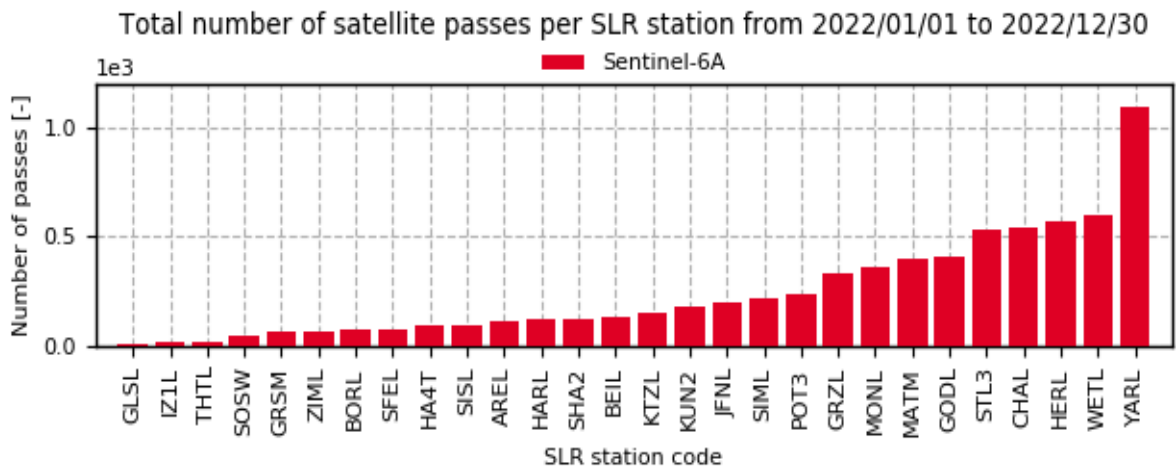
Figure 2-12: Total number of satellite passes per SLR station in 2022 (Sentinel-6A)
