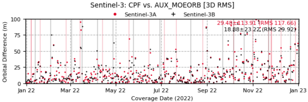
Figure 4-1: Orbital comparisons [3D RMS; m] between the Sentinel-3 CPF predictions and the Sentinel-3 CPOD STC products during 2022
