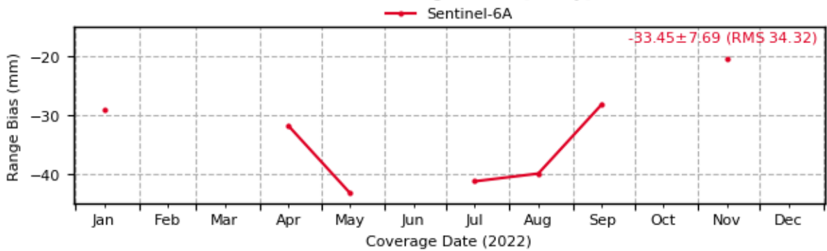
Sentinel-6: Evolution of Range Biases [1-way] (7824 - SFEL)
