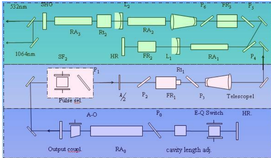
Figure 2. Diagram of Active-active mode-locked laser for LTT
