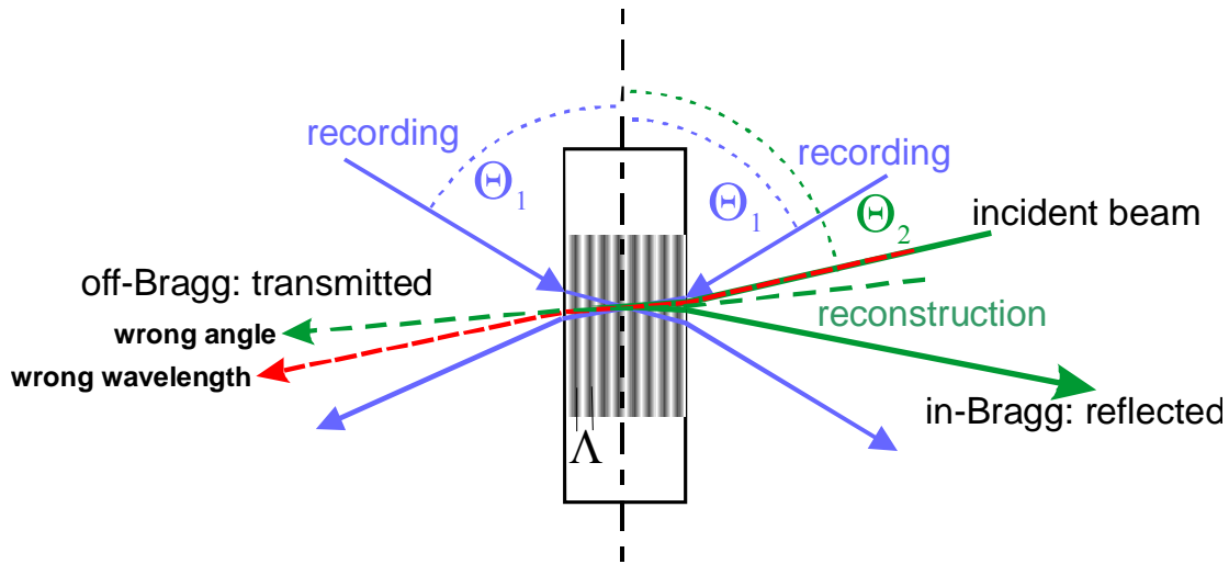
Figure 1. Optical layout of the recording and reconstruction of the holographic selector
