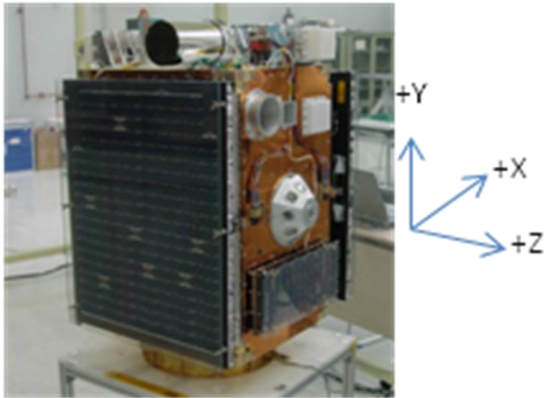
Figure 2. STSAT-2 Configuration
