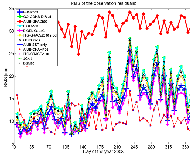
Figure 2: RMS of weekly LAGEOS solutions without OPR cross-track accelerations estimated (solution (b))
