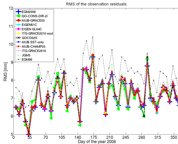
Figure 1: RMS of weekly LAGEOS solutions with the full set of OPR accelerations estimated (solution (a))
